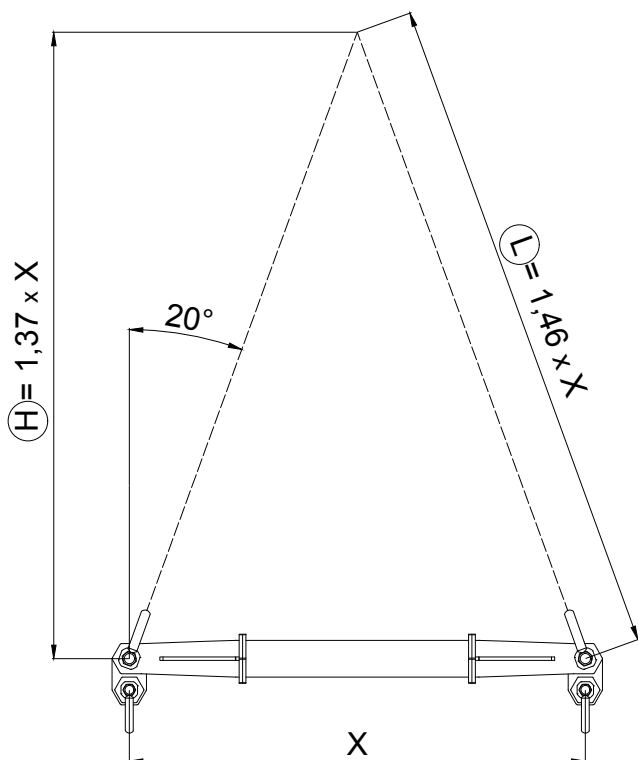
Dimensions at 20°
