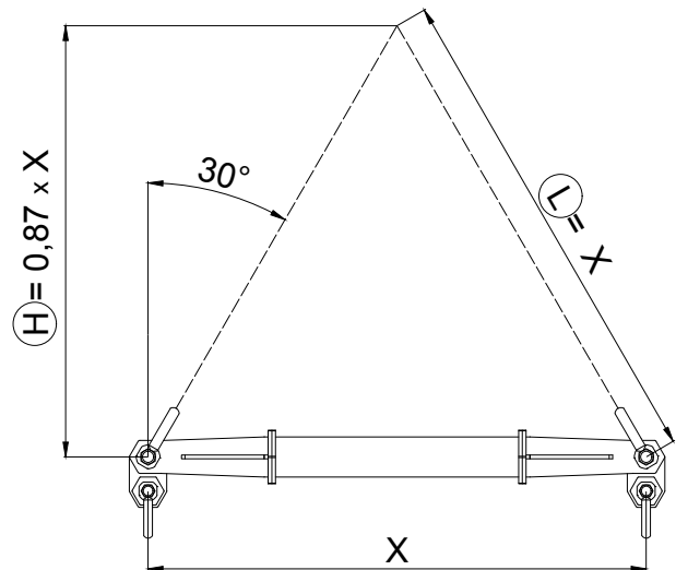
Dimensions at 30°
